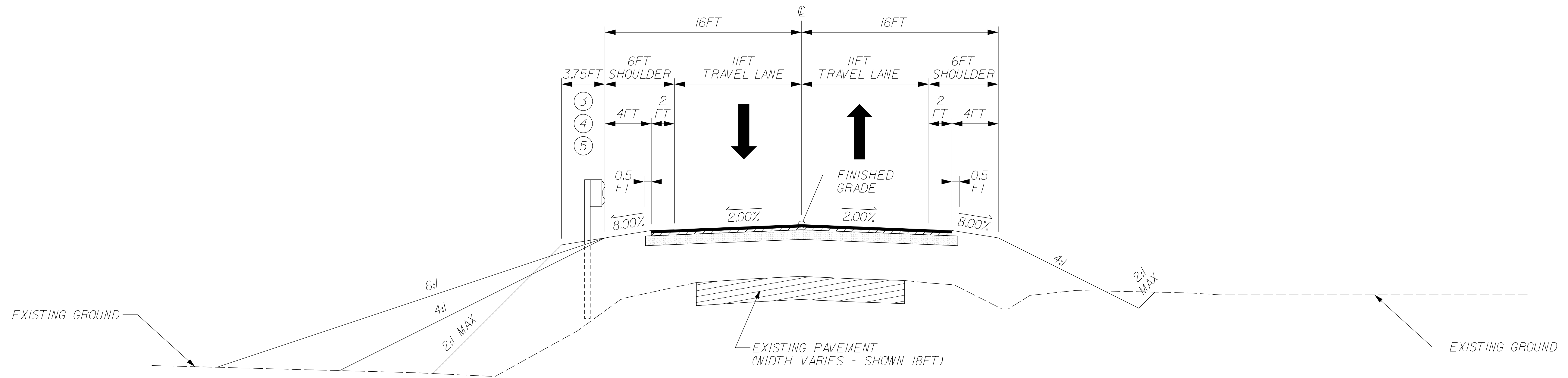
TYPICAL SECTION - ROADWAY SC 412 (RAINEY RD) FROM STA. 6+50.00 TO STA. 16+00.00
